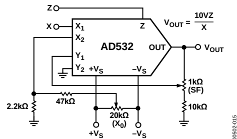
Figure 17. Divider Connection
