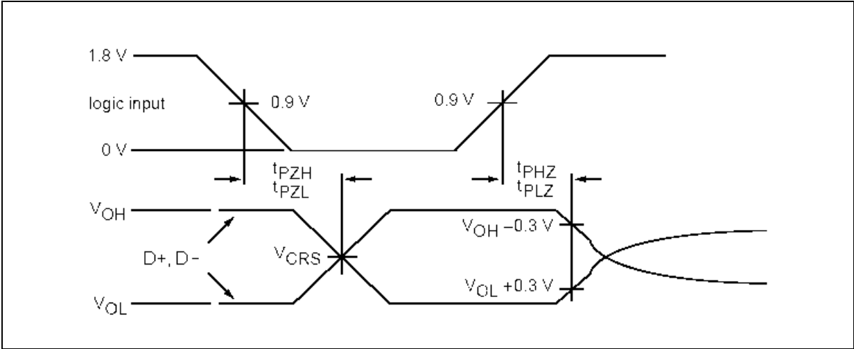
Figure 4. Turnaround time
