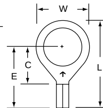
MU18-38R Stud Size 3/8 Wire Range 22-18
