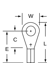
MU18-8R/L Stud Size 8 Wire Range 22-18
