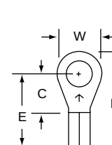
MU14-10R Stud Size 10 Wire Range 16-14
