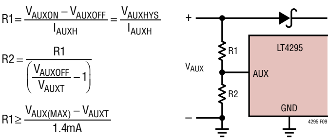
Figure 9. AUX Threshold and Hysteresis Calculation
