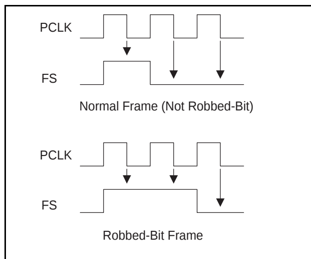
Figure 25 - Robbed-Bit Frame
