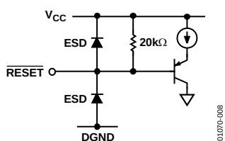
Figure 45. Reset Input
