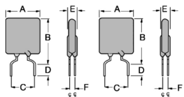
Fig.3 Lead Size : 20AWG Φ 0.81 mm Diameter
