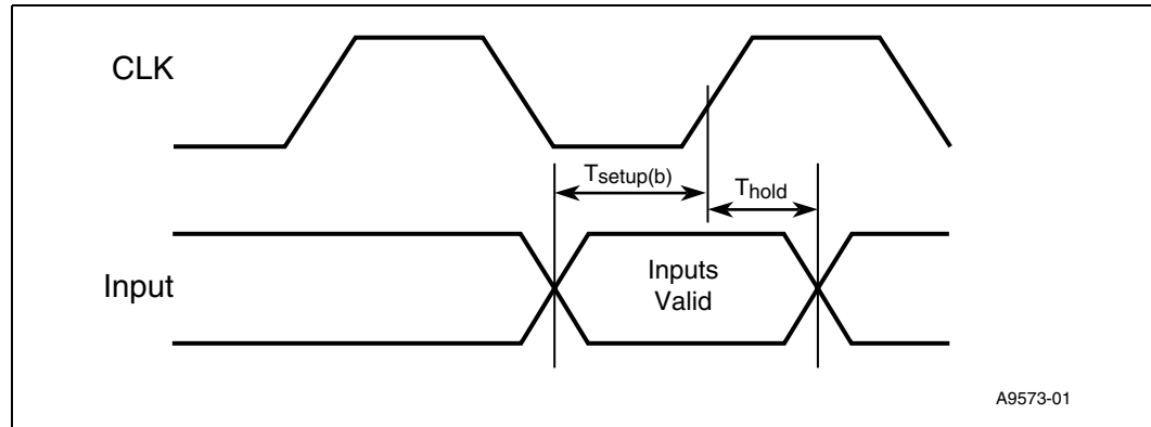
Figure 18. PCI Input Timing
