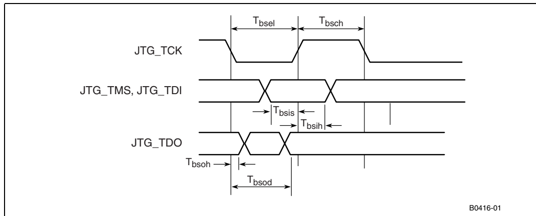
Figure 47. Boundary-Scan Reset Timings
