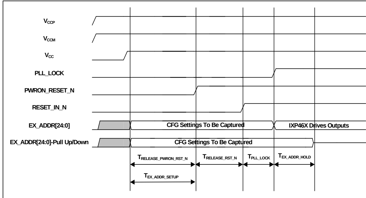
Figure 48. Reset Timings
