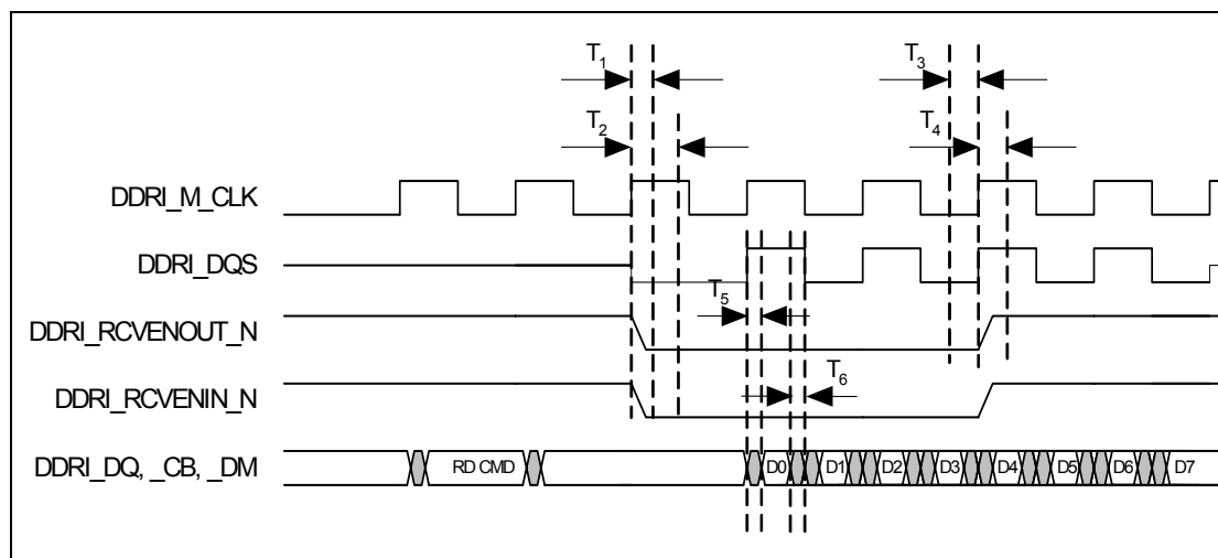
Figure 30. DDRI SDRAM Read Timings (2.0 CAS Latency)
