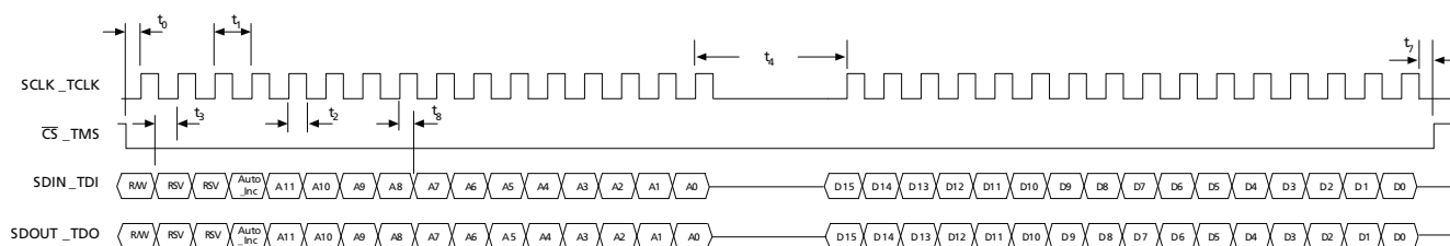
Figure 4-49: Write Mode
