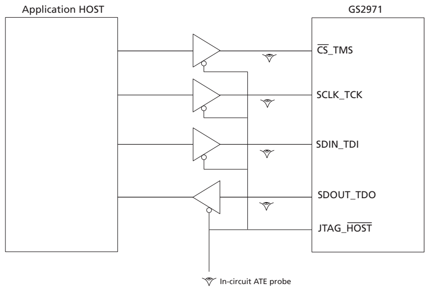
Figure 4-52: In-Circuit JTAG
