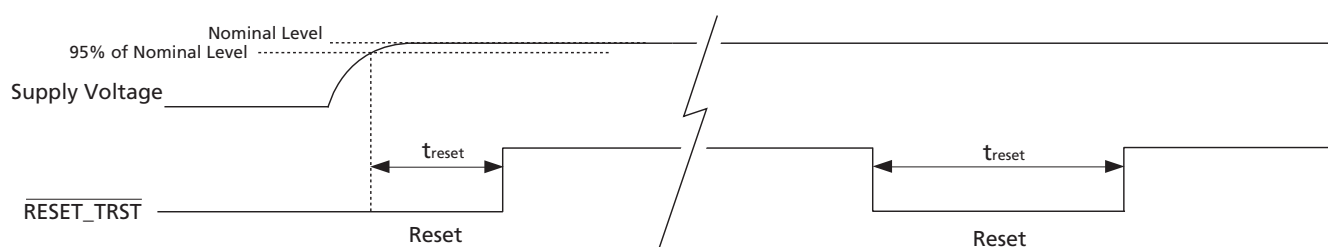
Figure 4-54: Reset Pulse
