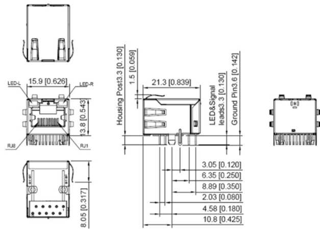
C: Tab up, w/ EMI Fingers
