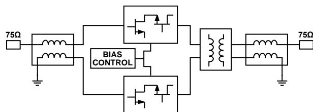
Figure 9. Simplified Schematic
