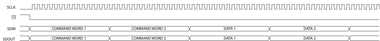
Figure 4-14: GSPI Write Timing—Auto-Increment with Loop-Through Operation (default)
