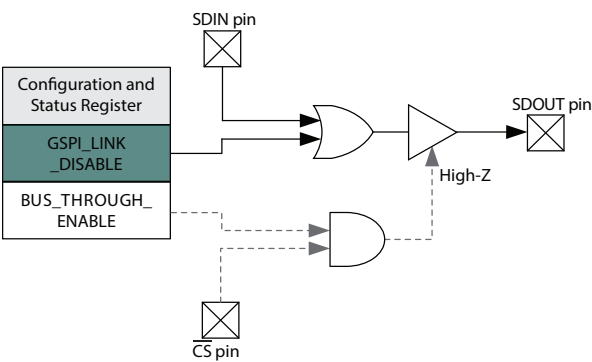
Figure 4-4: GSPI_LINK_DISABLE Operation
