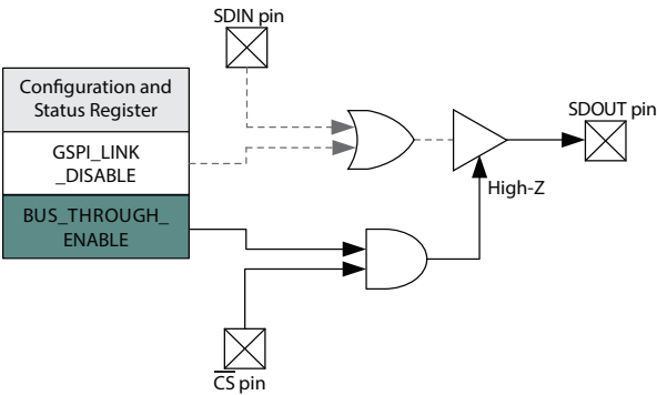
Figure 4-5: GSPI_BUS_THROUGH_ENABLE Operation
