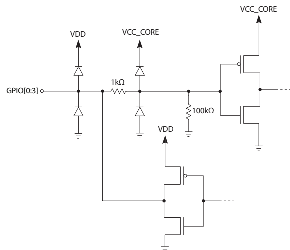
Figure 3-6: GPIO[0:3]
