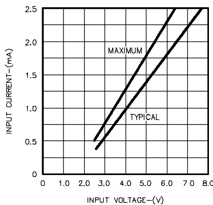
FIGURE 5. INPUT CHARACTERISTICS - SG2803
