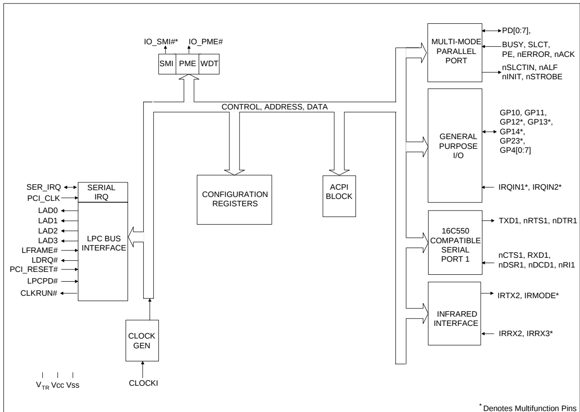
Figure 1 - LPC47N217 Block Diagram
