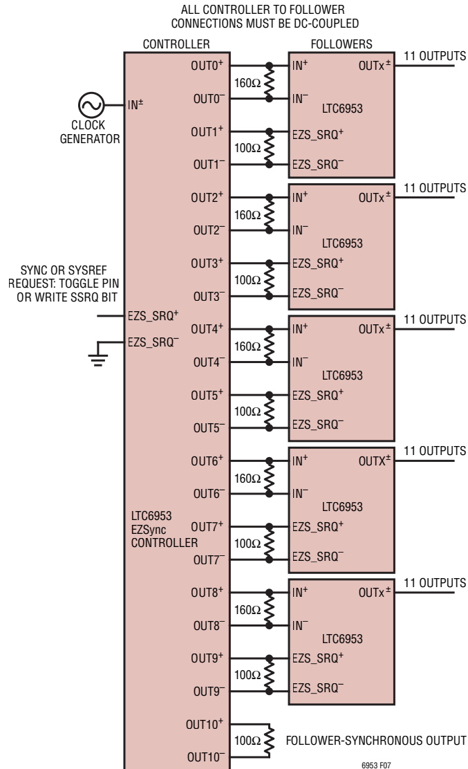
Figure 7. EZSync Multichip Synchronization with Request Pass-Through
