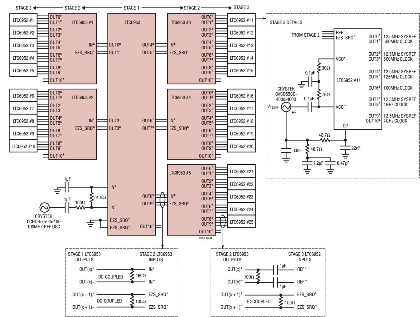
Generation of Up to 125 ADC Clock/SYSREF Pairs Using a Three-Stage Synchronization Architecture: Schematics
