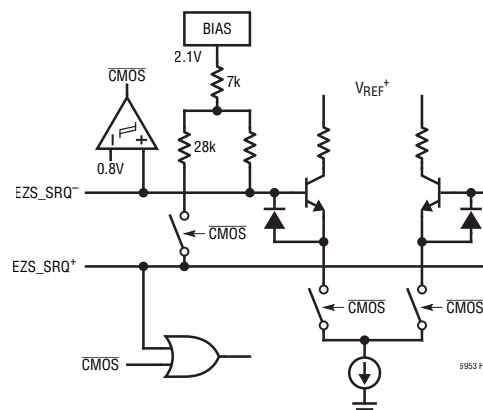
Figure 4. Simplified EZ_SRQ Interface Schematic
