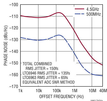
Cumulative Phase Noise, LTC6946 Driving LTC6953
