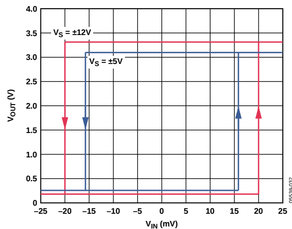
Figure 36. Comparator Hysteresis
