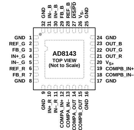
Figure 3. Pin Configuration
