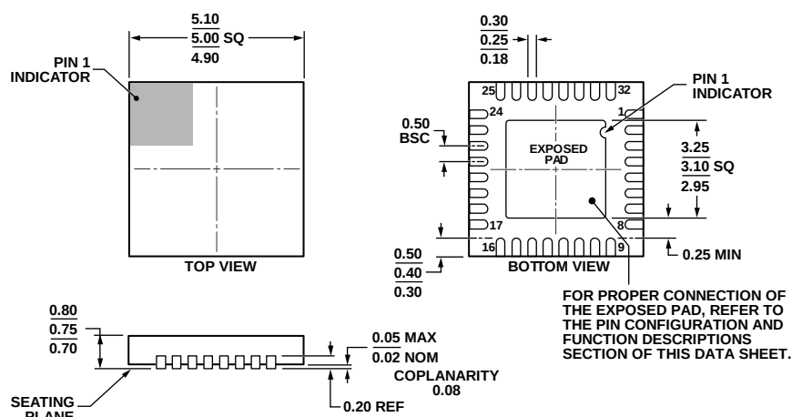
Figure 49. 32-Lead Lead Frame Chip Scale Package [LFCSP] 5 mm × 5 mm Body and 0.75 mm Package Height (CP-32-7)
