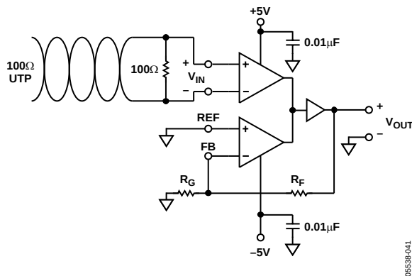
Figure 40. Differential-Mode Termination
